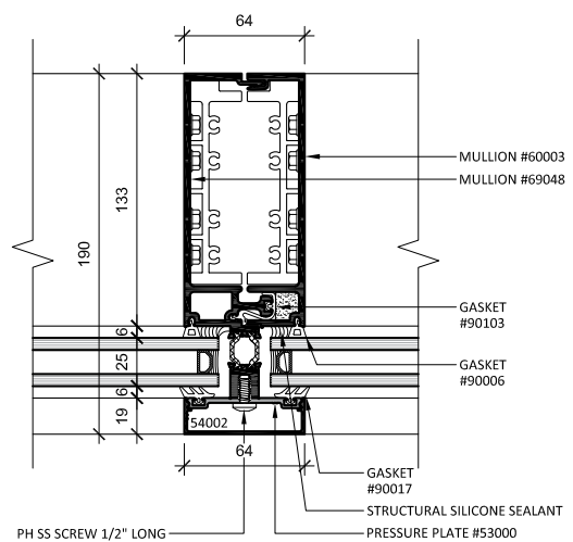
3 MULLION VISION SECTION
