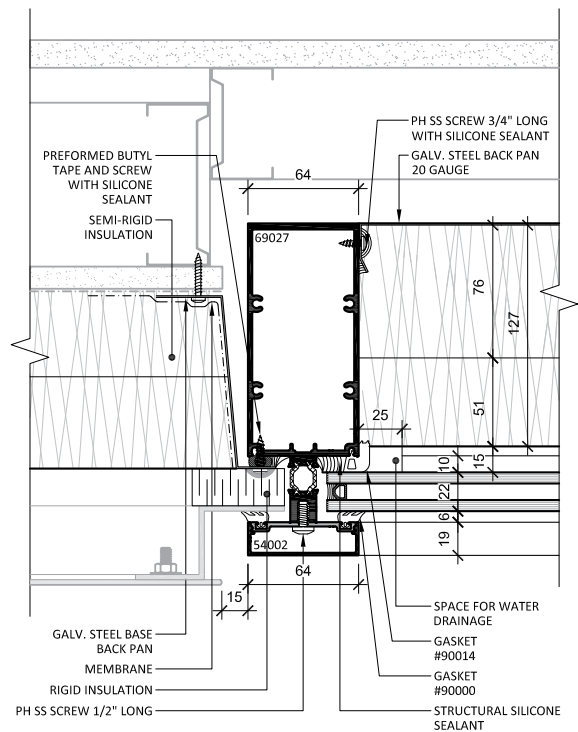
1 MULLION CONNECTED ELEMENTS SPANDREL PANEL
