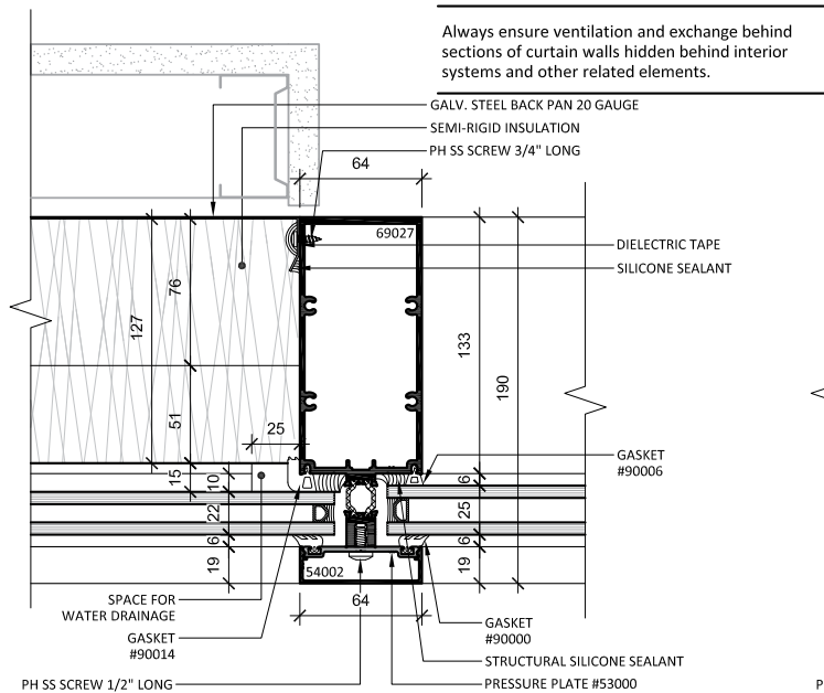
2 MULLION SPANDREL PANEL VISION SECTION
