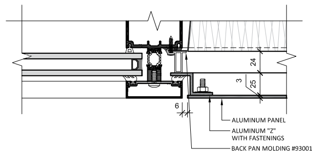
2 MULLION A2 ALUMINUM PANEL
