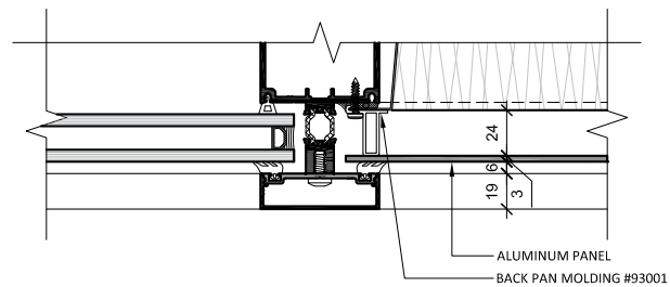
1 MULLION A1 ALUMINUM PANEL
