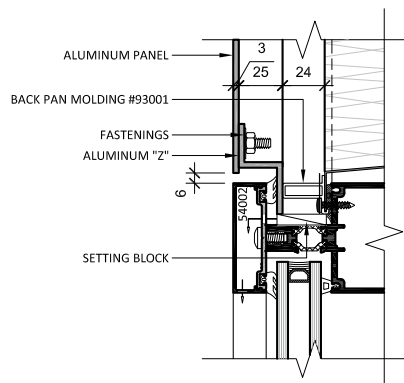
6 TRANSOM A2 ALUMINUM PANEL BASE
