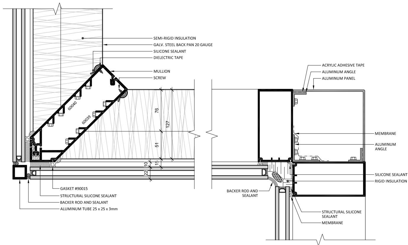
1 MULLION 90° OUTER CORNER STRUCTURAL SILICONE
