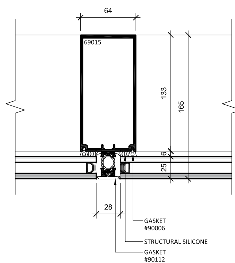
3 MULLION VISION SECTION
