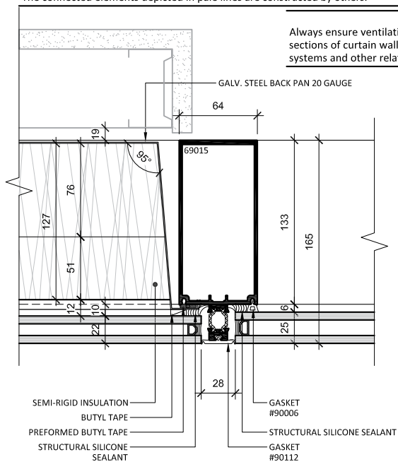
2 MULLION SPANDREL PANEL VISION SECTION
