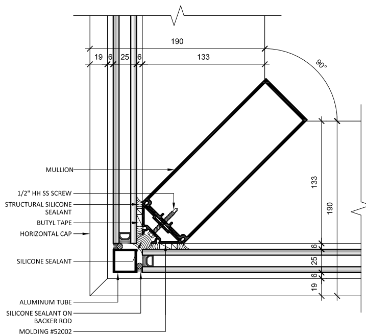
3 MULLION 90° OUTER CORNER STRUCTURAL SILICONE
