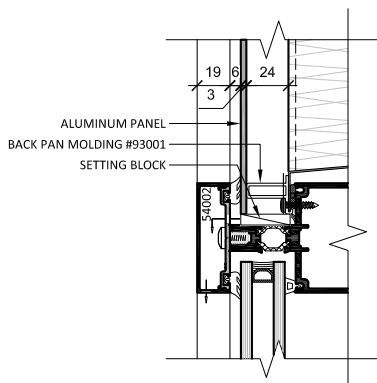
4 TRANSOM A1 ALUMINUM PANEL BASE
