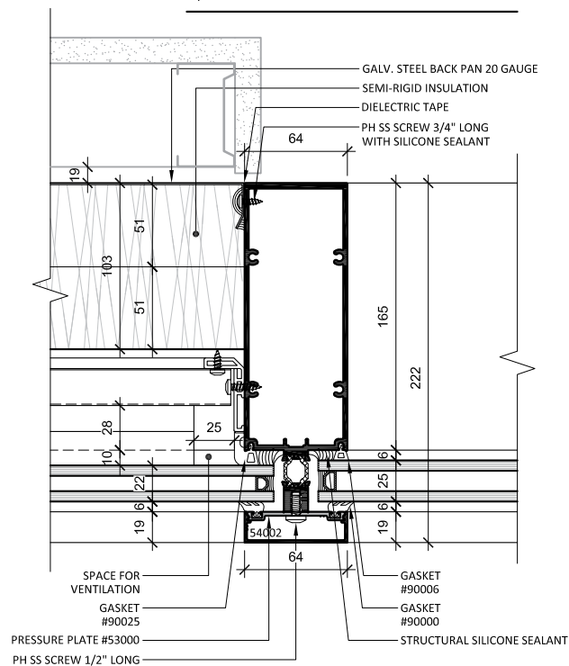
2 MULLION SHADOW BOX SECTION VISION SECTION
