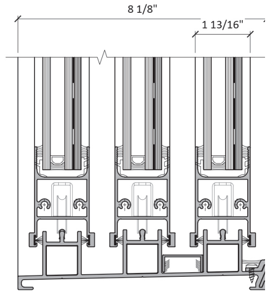
10 SILL DETAIL
