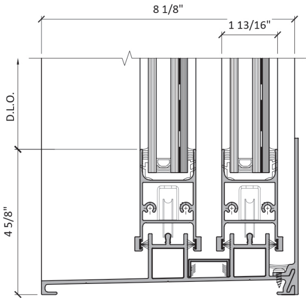
8 SILL DETAIL
