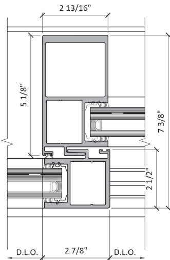
4 MEETING STILE
