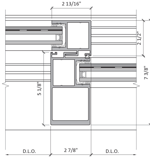
2 HEAVY DUTY MEETING STILE
