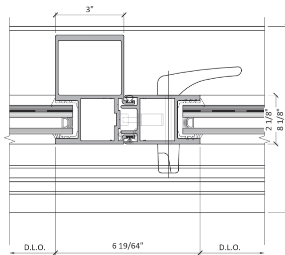
5 INTERLOCKING MEETING STILE
