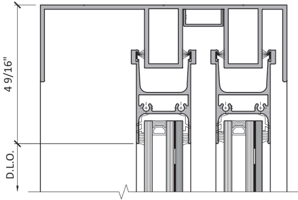
7 HEAD DETAIL
