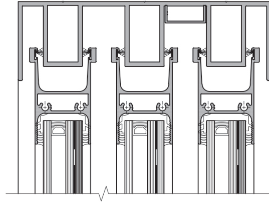
9 HEAD DETAIL
